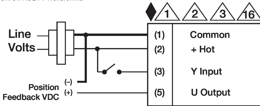
Floating Point AC 24 V Transformer (AC Only)
